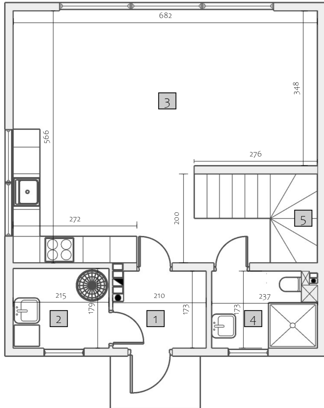
PARTER H= 280
