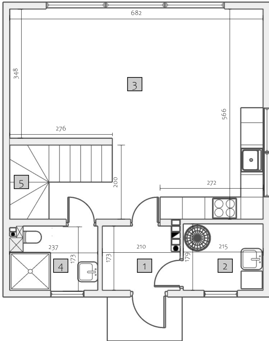
PARTER H= 280
